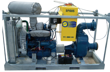
6" Centrifugal Pump
